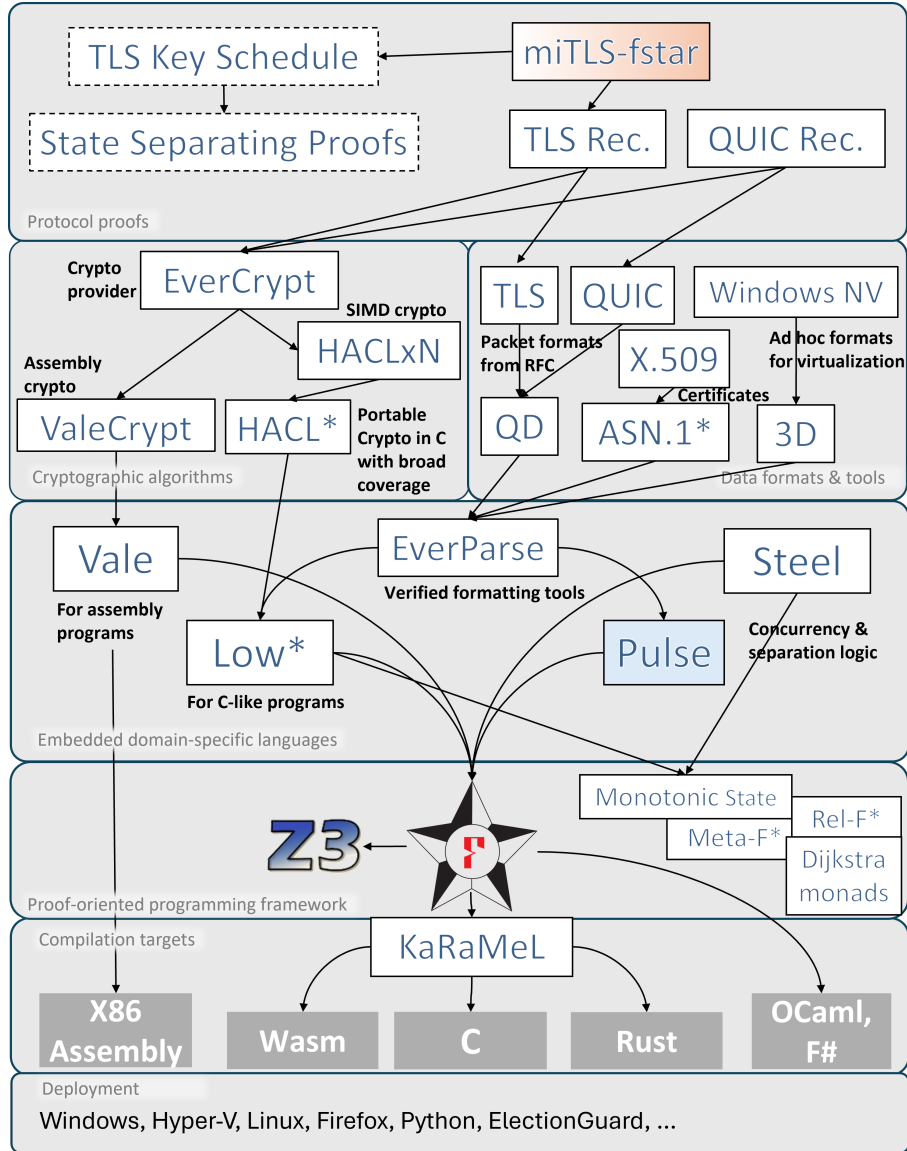
Figure 2: The Architecture of Project Everest , with arrows indicating dependencies among components. Z3 was developed independently. The TLS Key Schedule and State Separating Proofs are pen-and-paper formalizations. All the rest were implemented and proven correct in F*. Many tools and techniques continue to be developed within this same framework after Project Everest, e.g., Pulse. The proof of the TLS-1.3 handshake in miTLS-fstar was left incomplete, and, as such, is shown in a different color—however, recent advances [34] have resulted in a proof of security of a Rust implementation of TLS-1.3, building on Everest’s State Separating Proofs methodology, and via translation to a suite of proof tools, including F*.
